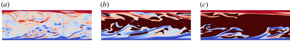
FIGURE 1. Contours of the instantaneous spanwise vorticity in the XY plane ( X horizontal and Y vertical axes). Dark colour represents the areas where the flow is not yielded. (a–c) Bi = 0, 1.4 and 2.1 . Colours scale from -3U_b/h (blue) to 3U_b/h (red).
