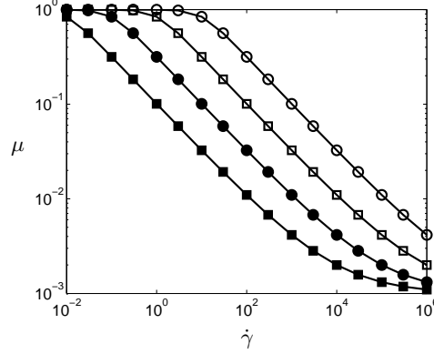
FIGURE 1. Viscosity \mu of Carreau-law model versus shear rate \dot{\gamma} for n = 0.5 , ( \circ ): \lambda = 0.1 , ( \square ): \lambda = 1 , ( \bullet ): \lambda = 10 , ( \blacksquare ): \lambda = 100
