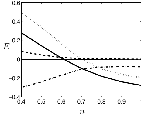
FIGURE 12. Integral of production and dissipation of perturbation kinetic energy E over the domain for a fixed \lambda = 10 and Reynolds number=20. (— · — ·): Dissipation, (...): Production, (— — —): shear-thinning production and (—): sum
