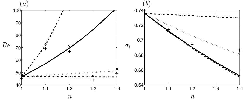
FIGURE 16. (a) Neutral curves and (b) Frequency of the least stable mode for shear-thickening cylinder flow, (---): \lambda = 0.1 , (...): \lambda = 1 , (—): \lambda = 10 and (— — —): \lambda = 100 . Symbols indicate results from the direct numerical simulations: (+) : unstable cases & (x) : stable cases.
