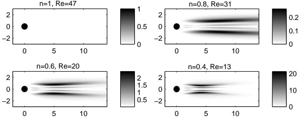
FIGURE 14. Spatial distribution of the additional production of perturbation kinetic energy, -\frac{2}{Re}A|e_{ij}E_{ij}|^2 , for a fixed \lambda = 10 along the neutral curve-normalized by the energy of perturbation.
