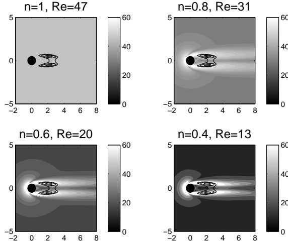
FIGURE 10. Spatial distribution of the local Reynolds number along the neutral curve for \lambda = 10 and values of n listed on each plot. The contour lines represent the regions of largest structural sensitivity.
