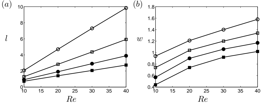
FIGURE 5. (a) Bubble length l , and (b) Bubble width w for fixed \lambda = 10 , ( \circ ): n = 0.4 , ( \square ): n = 0.6 , ( \bullet ): n = 0.8 , ( \blacksquare ): n = 1
