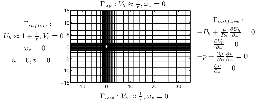
FIGURE 2. Mesh used for the present simulations; only one out of eight lines passing through the pressure nodes is drawn for clarity. The boundary conditions pertaining the outer boundary are also reported for base flow and perturbation. Zero velocity is imposed at the surface of the cylinder.
