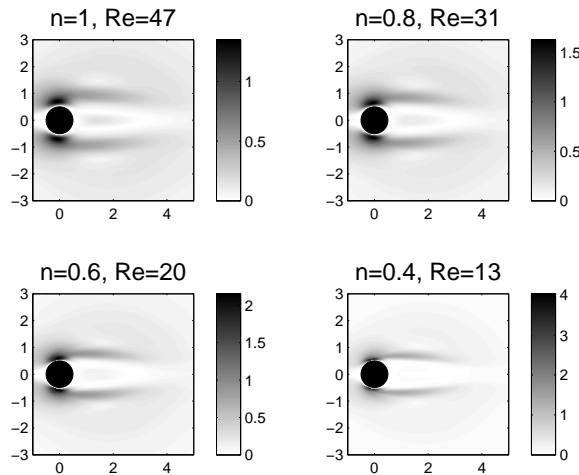
FIGURE 11. Sensitivity map due to base-flow modifications for a fixed \lambda = 10 along the neutral curve
