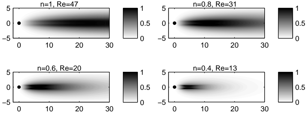
FIGURE 7. Unstable global modes: Spatial distribution of the velocity field modulus at the critical Reynolds number for fixed \lambda = 10 and for 4 values of n .
