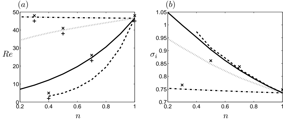
FIGURE 3. (a) Neutral curves Re (b) Frequencies \sigma_i - Linear Instability Analysis, (- . - .) : \lambda = 0.1 , (...) : \lambda = 1 , (-) : \lambda = 10 & (- - -) : \lambda = 100 and Direct Numerical Simulation, ( \times ) : unstable cases and ( + ) : stable cases
