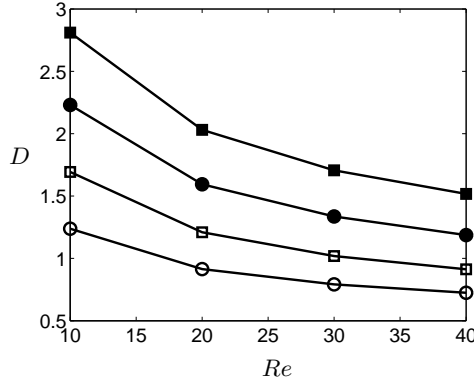
FIGURE 6. Drag coefficient, D , versus the Reynolds number, Re , for \lambda = 10 , ( \circ ): n = 0.4 , ( \square ): n = 0.6 , ( \bullet ): n = 0.8 , ( \blacksquare ): n = 1
