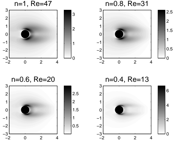
FIGURE 8. Spatial distribution of the magnitude of the adjoint global mode at the critical Reynolds number for a fixed \lambda = 10 for 4 values of n .
