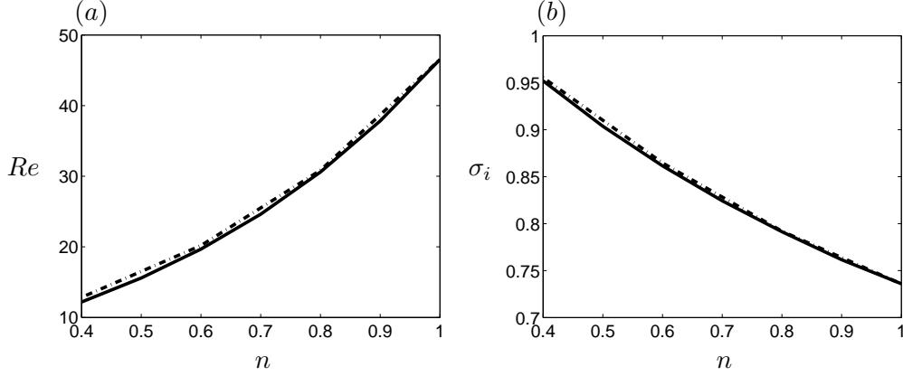
FIGURE 15. Effect of the viscosity disturbance in the perturbation equations. (a) Neutral stability curve and (b) frequencies of the least stable mode at critical conditions for \lambda = 10 . (—): including viscosity disturbance, (---): excluding viscosity disturbance.
