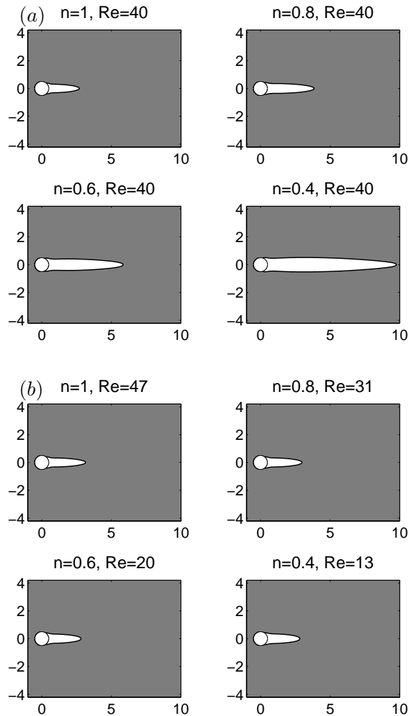
FIGURE 4. Visualization of the recirculation bubble behind the cylinder for different values of the exponent n . (a) Re = 40 and \lambda = 10 , (b) critical values of the Reynolds number for fixed \lambda = 10 .
