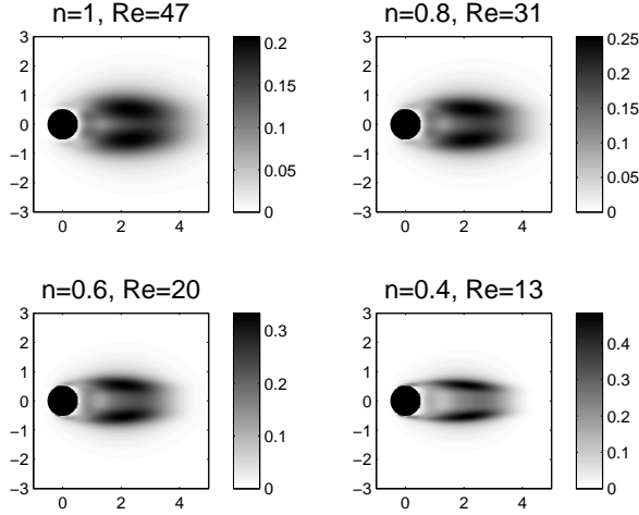
FIGURE 9. Sensitivity map for a fixed \lambda = 10 along the neutral curve
