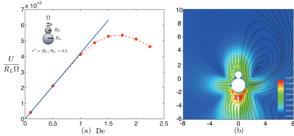
FIG. 2. Demonstration of snowman locomotion. In the case r^* = R_U/R_L = 0.5 and \zeta = 0.5 , we plot: (a) dimensionless propulsion speed, U/R_L\Omega , as a function of the Deborah number, De . (Red dots and dashed line: numerical simulations in an Oldroyd-B fluid; blue solid line: theoretical calculation using the reciprocal theorem in a second-order fluid, Eq. (36).) (b) The streamline pattern and speed (shaded/color map) of the secondary flow for De = 0.1 (streamline patterns at higher De are qualitatively similar).
