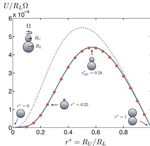
FIG. 3. Propulsion speed of snowman with two touching spheres as a function of the ratio of radii at \text{De} = 0.1 and \zeta = 0.5 . Red dots: numerical results in an Oldroyd-B fluid. Blue solid line: theoretical calculation for second-order fluid. Black dotted line: simplified analytical model (Eq. (51)).
