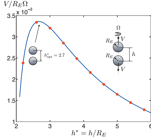
FIG. 6. Dimensionless repulsion speed, V/R_E\Omega , of two equal co-rotating spheres as a function of their dimensionless separation distance, h^* , at De = 0.1 and \zeta = 0.5 . Red dots: numerical results in an Odroyd-B fluid. Blue solid line: theoretical calculation for a second-order fluid.
