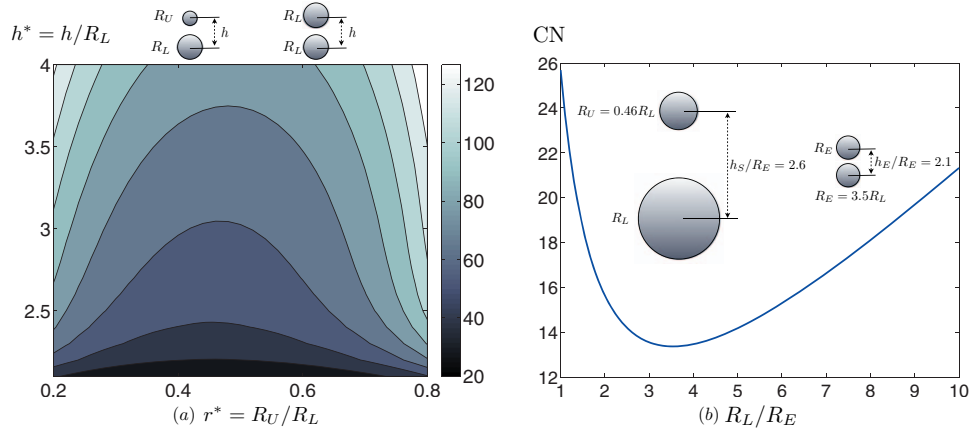
FIG. 7. (a) Condition number (CN) for the matrix \mathbf{C} as a function of sphere size ratio ( r^* ) and dimensionless separation distance ( h^* = h_S^* = h_E^* ). (b) CN as a function of R_L/R_E , for r^* = 0.46 , h_S^* = 2.6 , and h_E^* = 2.1 .
