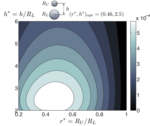
FIG. 5. Optimization snowman propulsion. Isovalues of the dimensionless propulsion speed with dimensionless separation distance, h^* , and ratio of sphere radii, r^* . The optimal geometry for maximum propulsion speed is given by (r^*, h^*)_{\text{opt}} = (0.46, 2.5) . A schematic diagram showing the optimal geometry is drawn to scale above.
