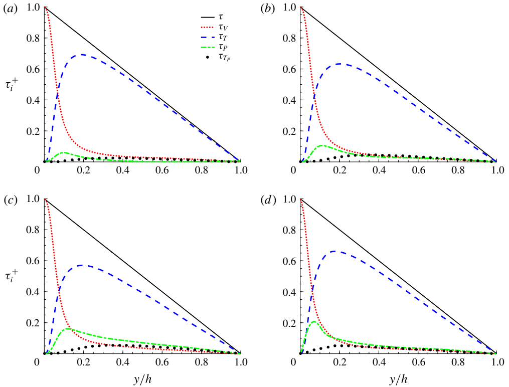
FIGURE 7. (Colour online) Momentum budget, normalized with \rho_f U_*^2 , for oblate particles at (a) \phi = 5\% , (b) \phi = 10\% and (c) \phi = 15\% , and for spheres at (d) \phi = 10\% . Here, \tau is the total stress, \tau_V denotes viscous stress, \tau_T = -\langle u'_c v'_c \rangle the turbulent Reynolds shear stress of the combined phase and \tau_p the particle-induced stress. The particle Reynolds shear stress \tau_{Tp} = -\langle u'_p v'_p \rangle is also depicted with dots.
