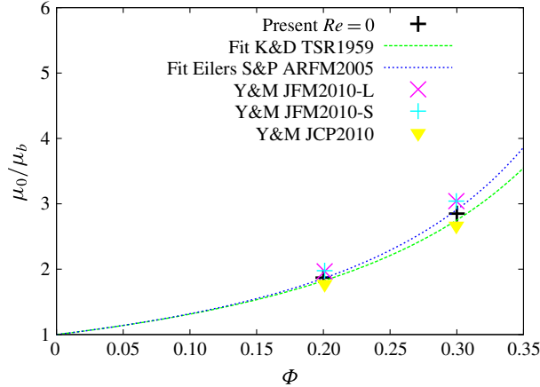
FIGURE 1. (Colour online) Relative viscosity \nu_r versus the volume fraction \Phi in a Couette flow in absence of inertia, Re = 0 . The present data are compared with the results by Yeo & Maxey (2010a,b) and the Eilers fit ( 1 + 1.25\Phi/(1 - \Phi/0.65) ).
