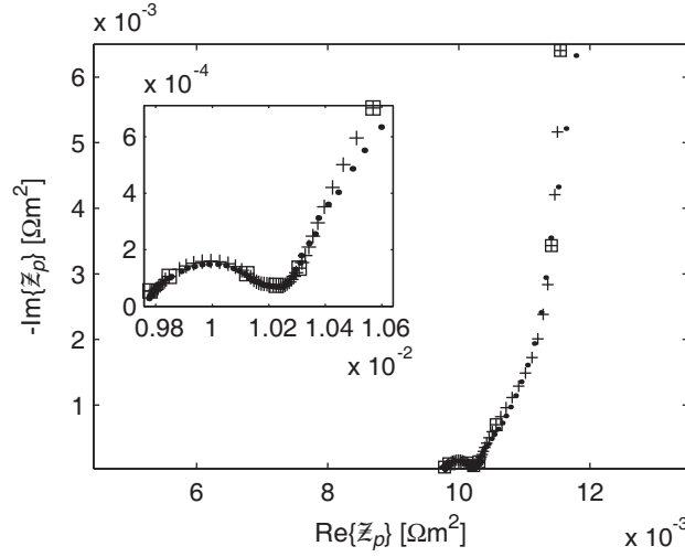
Figure 4.2: Spectra of the experimental (●) and the fitted (+) impedances of a fresh \text{Li}_x\text{Ni}_{0.8}\text{Co}_{0.15}\text{Al}_{0.05}\text{O}_2 positive porous electrode at a state of charge corresponding to x = 0.43 ; f = 1000, 125, 10, 1, 0.1, 0.01, 0.001 and 0.0005 Hz marked with □.
