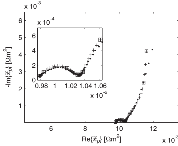
Figure 4.1: Spectra of the experimental (●) and the fitted (+) impedances of a fresh \text{Li}_x\text{Ni}_{0.8}\text{Co}_{0.15}\text{Al}_{0.05}\text{O}_2 positive porous electrode at a state of charge corresponding to x = 0.54 ; f = 1000, 125, 10, 1, 0.1, 0.01, 0.001 and 0.0005 Hz marked with □.
