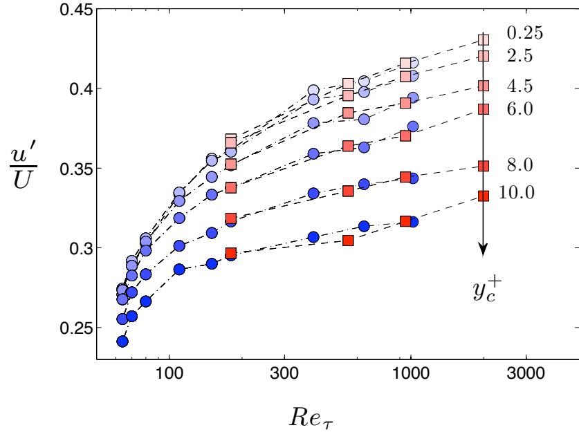
FIGURE 11. Relative turbulence intensity, u'/U , as function of the friction Reynolds number at different (approximate) wall positions, y_c^+ , for channel flows: \bullet (Tsukahara et al. 2005; Kawamura et al. 1999; Abe et al. 2004) and \blacksquare (del Álamo & Jiménez 2003; del Álamo et al. 2004; Hoyas & Jiménez 2006).
