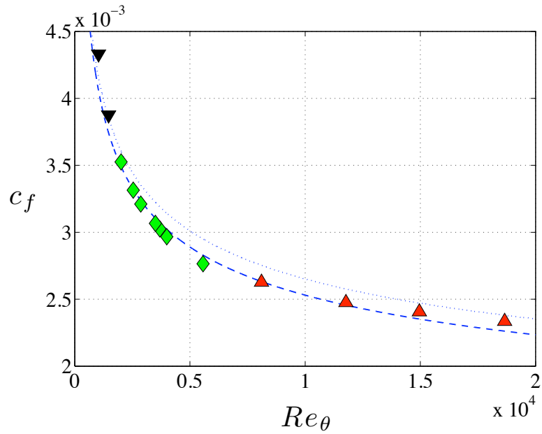
FIGURE 25. Skin friction coefficient, c_f , vs. Re_\theta . Tripping configuration A: \blacktriangle , B: \blacklozenge and C: \blacktriangledown . Coles-Fernholz relation with coefficients determined by Nagib et al. (2007) ( \kappa = 0.384 & C = 4.127 ): - -, and with classical values ( \kappa = 0.41 & C = 5.0 ): \cdots .
