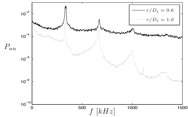
FIGURE 5. Power-spectral density function of the streamwise velocity component measured behind the inner ( r/D_i = 0.6 ) and outer ( r/D_i = 1.0 ) wall at U_o = 8 m/s, r_u = 1 and x/D_i = 0.5 for the thick wall.
