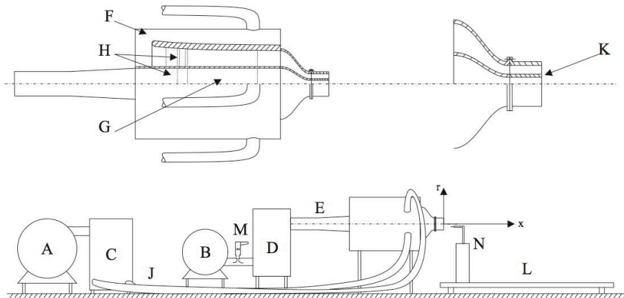
FIGURE 4.7. Schematic of the Coaxial Air Tunnel (CAT) facility at the University of Bologna. A ) outer jet blower, B ) inner jet blower, C ) outer jet pre-settling chamber, D ) inner jet pre-settling chamber, E ) inner jet diffuser, F ) outer jet settling chamber, G ) inner jet settling chamber, H ) screens and honeycombs, J ) outer jet hoses, K ) close-up of the jet exit with the thick separating wall, L ) axial traversing, M ) heat gun, and N ) radial traversing.
