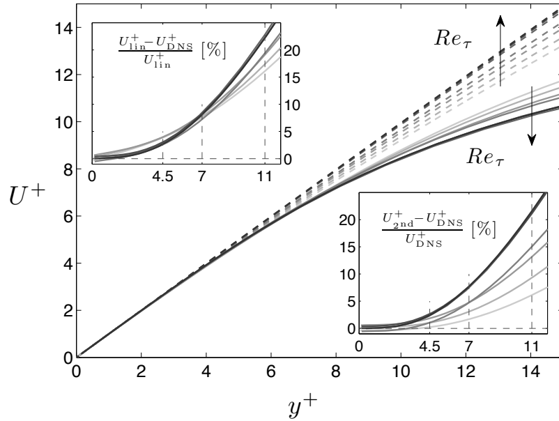
FIGURE 9. Mean streamwise velocity profile in inner scaling for channel flow with Re_\tau = 64, 80, 110, 150, 395, 640, and 1020 from DNS (—) (Tsukahara et al. 2005; Kawamura et al. 1999; Abe et al. 2004) and equation (2) to second order (- - -). The relative deviation of the linear profile without and with the second order term from the DNS is depicted in the upper and lower insert, respectively. Profiles and error curves with increasing Re_\tau are shown in progressively darker shades of gray.
