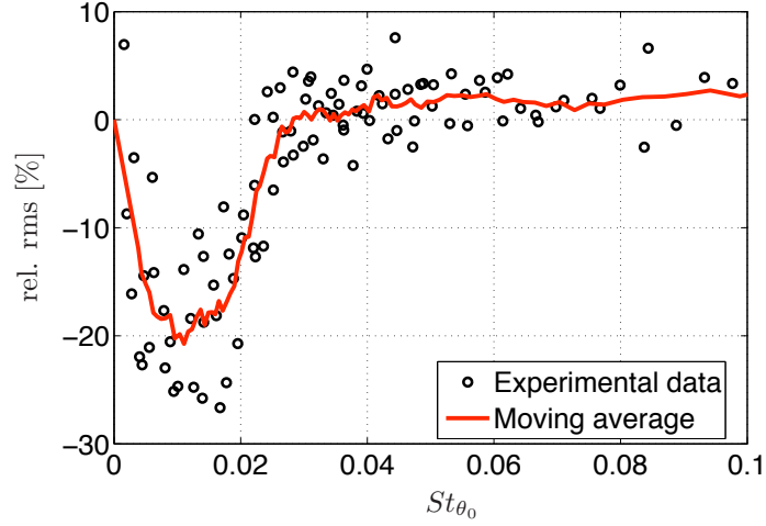
FIGURE 4. Relative change in streamwise velocity rms at x/D = 3 between excited and unexcited case for different exit velocities.
