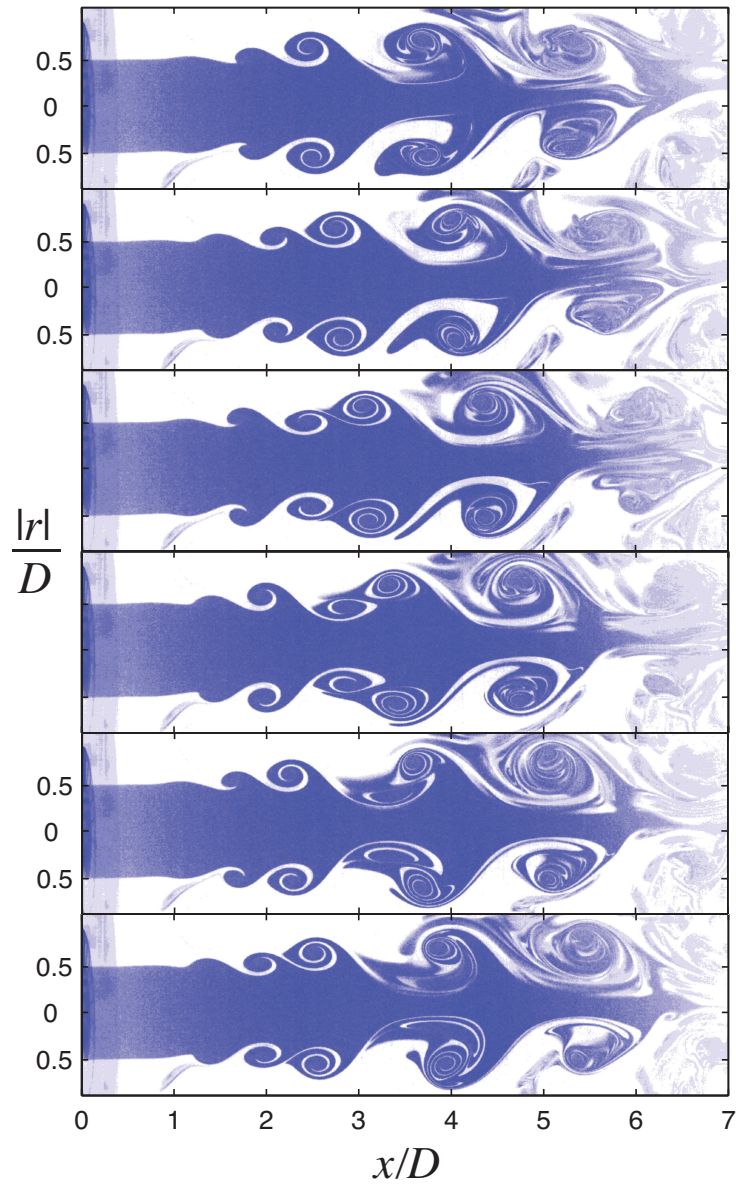
FIGURE 2.2. Flow visualisation of the centreline evolution of an axis-symmetric air jet with Re_D \approx 5000 issuing into air at rest. Subsequent snapshots are ordered from top to bottom with a time interval of 5 ms.
