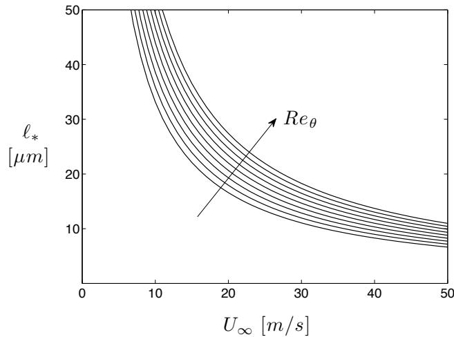
FIGURE 9. Variation in the viscous length scale, l_* , as function of the free stream velocity, U_\infty , for various Reynolds numbers. The functional relationship between all three quantities was computed using the Coles-Fernholz relation, eq. (13). (cf. section 5.1), with the constants established by Nagib et al. (2007). The Reynolds number shown represent Re_\theta \times 10^{-3} = 1, 2, 4, \dots, 256 .
