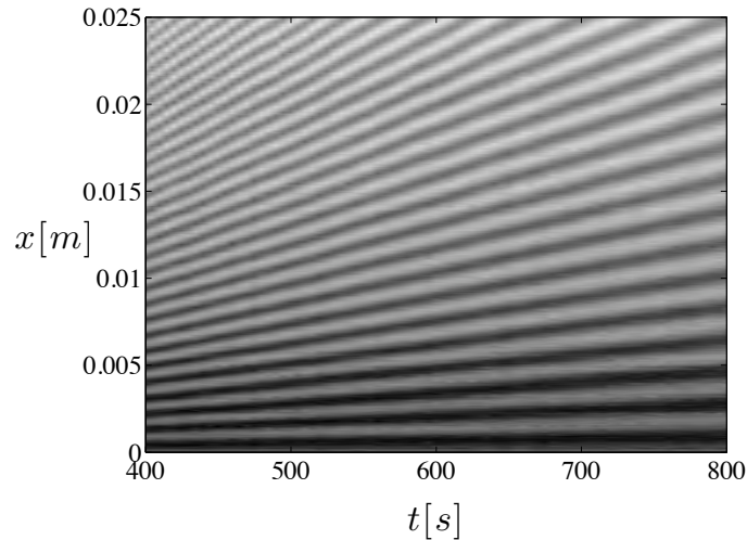
FIGURE 4. x - t diagram as extracted from a time series of fringe pattern images for the case shown in figure 3 after reaching steady conditions. Note that the shown pattern was extracted from a region, where the distortion by dust particles has diminished.
