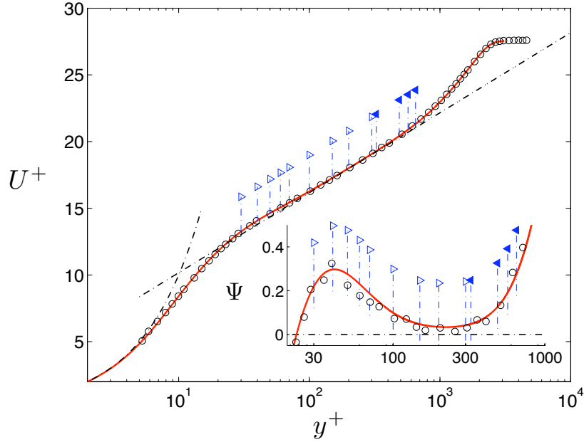
FIGURE 3.4. Schematic of the logarithmic region according to various sources. \circ : ZPG TBL experiments by Örlü (2009a) at Re_\theta = 8105 . - : Composite profile by Chauhan et al. (2009), \triangleright & \triangleleft : begin & end of logarithmic region (cf. table 1). Deviation from the log law, \Psi , is depicted in the insert. The linear and logarithmic profile with \kappa = 0.384 and B = 4.17 is indicated through the dash-dotted lines.
