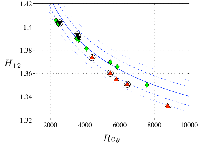
FIGURE 14. Shape factor, H_{12} , vs. Re_{\theta} . Tripping configuration A: \blacktriangle , B: \blacklozenge and C: \blacktriangledown . Integration of composite profile (Chauhan et al. 2009), H_{num} : —, H_{num} \pm 0.008 : - -, H_{num} \pm 1\% H_{num} : ··.
