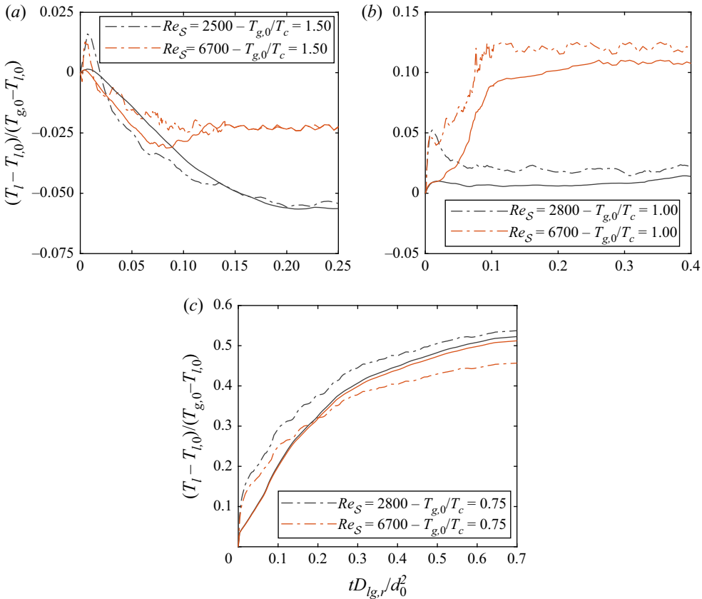
Figure 8. Dimensionless liquid temperature at the interface (T_{l,r} - T_{l,0})/(T_{g,0} - T_{l,0}) (dotted line) and average liquid temperature (T_{l,v} - T_{l,0})/(T_{g,0} - T_{l,0}) (continuous line) at (a) T_{g,0}/T_c = 1.5 , (b) T_{g,0}/T_c = 1.0 and (c) T_{g,0}/T_c = 0.75 .
