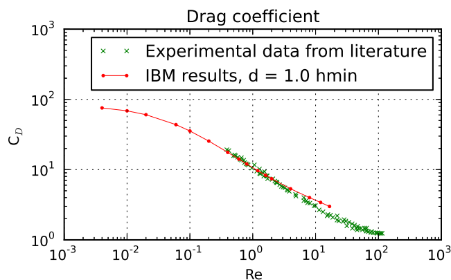
FIGURE 4.4. Direct numerical simulations of a flow over one Lagrangian point for various Reynolds numbers. The diameter of the model cylinder d is set to one mesh spacing h_{\min} . For comparison, literature data from Tritton (1959) is given.
