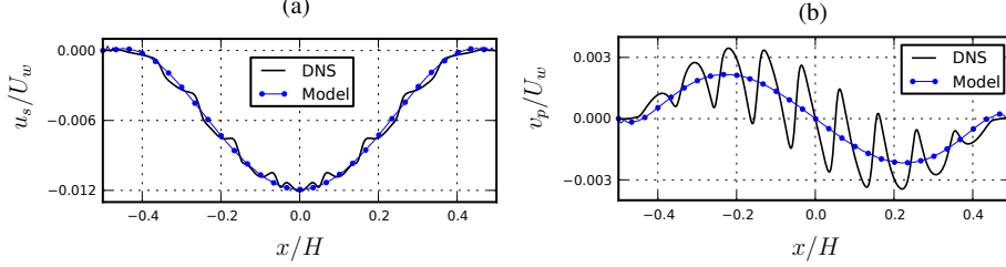
FIGURE 4.2. Results of the lid-driven cavity problem using direct numerical simulation and homogenised model for porous material. In frame (a), we show slip velocity and in frame (b), we show penetration velocity. Both velocities are sampled at coordinate y = 0.01 H . Volume fraction of solid material is 2 % and scale separation parameter is l/H = 0.1 .
