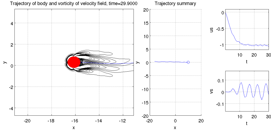
FIGURE 3.9. Results of a cylinder with velocity difference imposed at the top and the bottom, producing a jet that moves it forward. On the left, the vorticity field is shown at the end of the simulation. In the middle, the trajectory line is drawn. On the right, time statistics of the horizontal cylinder velocity u_s and the vertical cylinder velocity v_s are shown.
