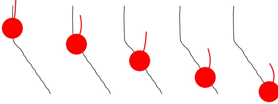
FIGURE 3.6. Results of freely falling cylinder with elastic filament clamped behind it. The length of the filament is L = 1.0 D . The body is shown at five different time instances. The free-fall trajectory is shown by the black line, which is not in scale with the body.
