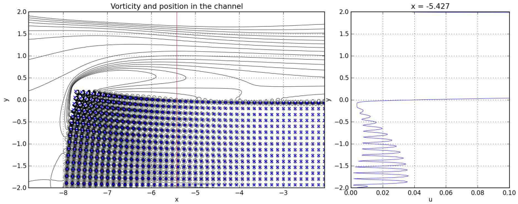
FIGURE 4.5. IB simulations of a flow over a poroelastic obstacle in a two-dimensional channel. The Reynolds number based on the channel height is around 100, and the solid volume fraction is around 1%. On the left, we show vorticity of the flow and the final shape of the obstacle. On the right, we show the stream-wise velocity profile along the slice marked by the red line.
