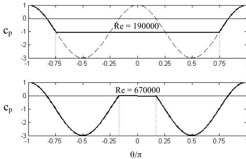
Figure 3.2 c_p = (p(\theta) - p_\infty) / \frac{1}{2} \rho U_\infty^2
